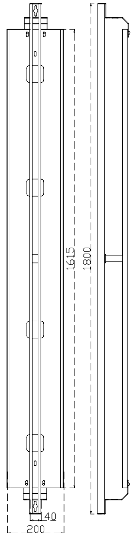
M-AC-018/55 * 1800 mm
