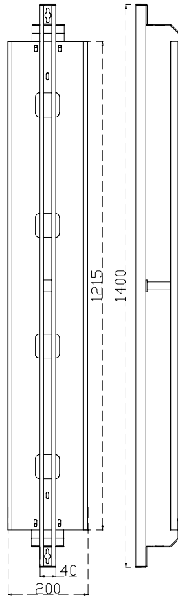
M-AC-014/55 * 1400 mm
