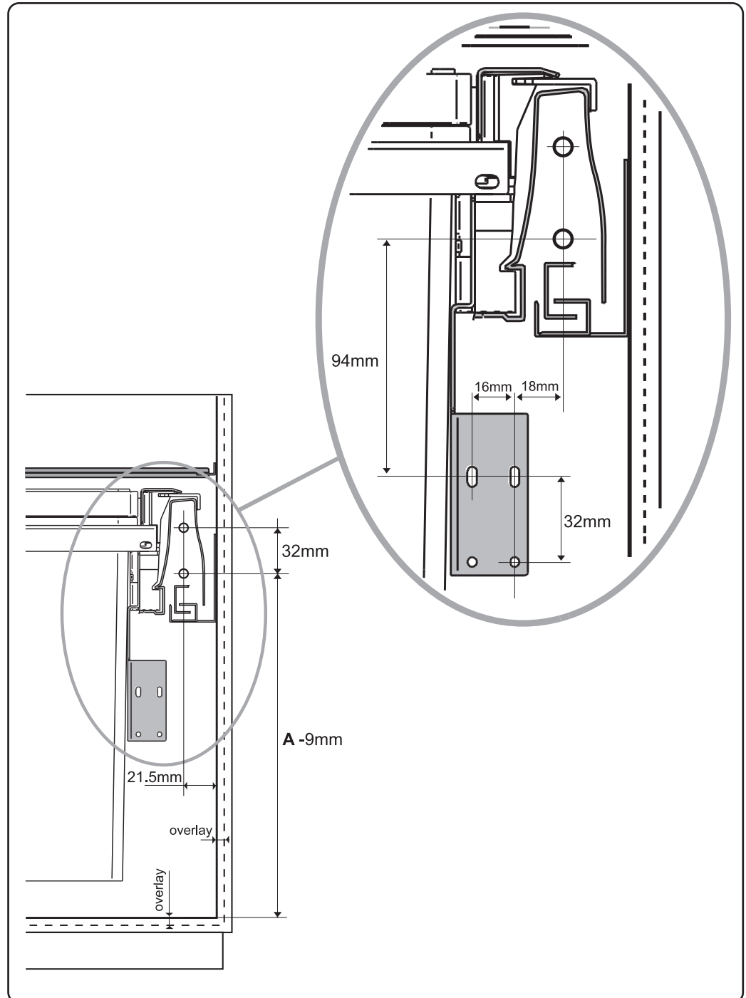
Grass DWD XP drawer front drilling position
